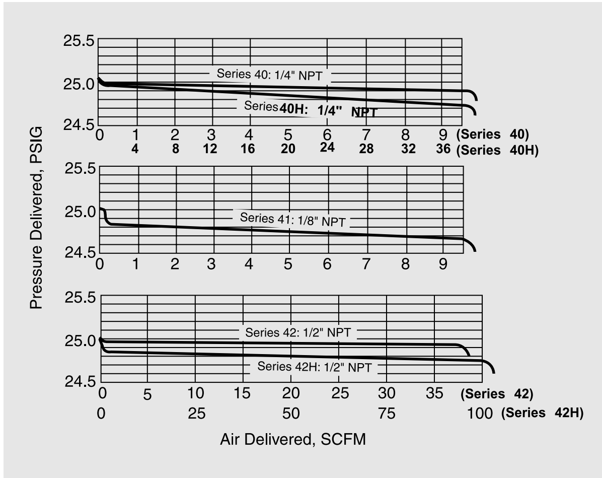
Graph 1 Droop Effect
