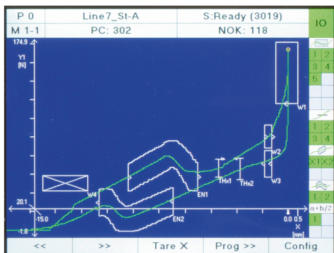
Figure: Measurement window M1-1 contains a graph of the measurement curve. Shows a curve containing a forward and return section and detailed evaluation using windows, envelopes, thresholds and mathematical operations.
