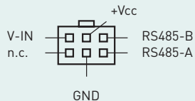
Molex socket 6-pin (f)
