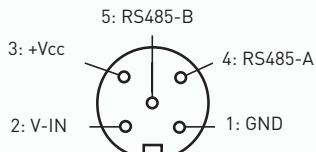
M12/5-pin (f)
